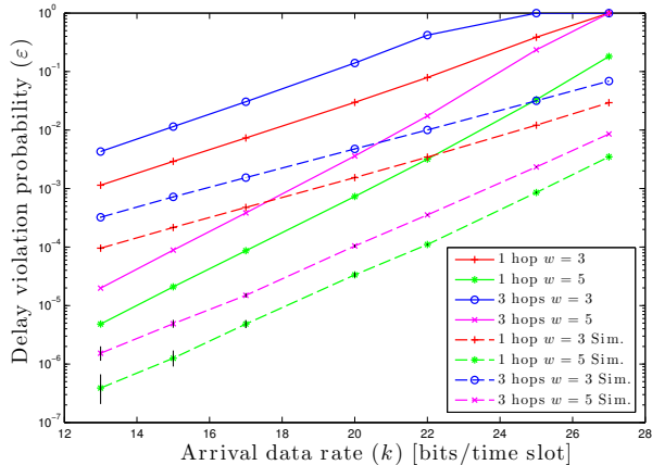
Fig. 2. Analytical delay bound and simulation results for a path consisting of one link with average SNR of 5 dB and a path consisting of 3 links with average SNR of 5, 10 and 7 dB. The target delay is w = \{3, 5\} time slots.
