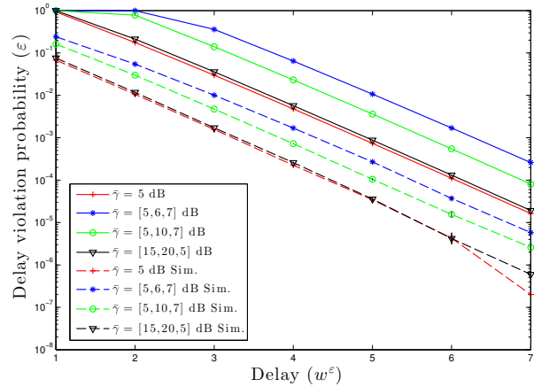
Fig. 3. Three 3-hop paths having the same bottleneck link are compared to one another and to a 1-hop path regarding both the analytical bound and simulation results. The arrival data rate is k = 20 bits per time slot.
