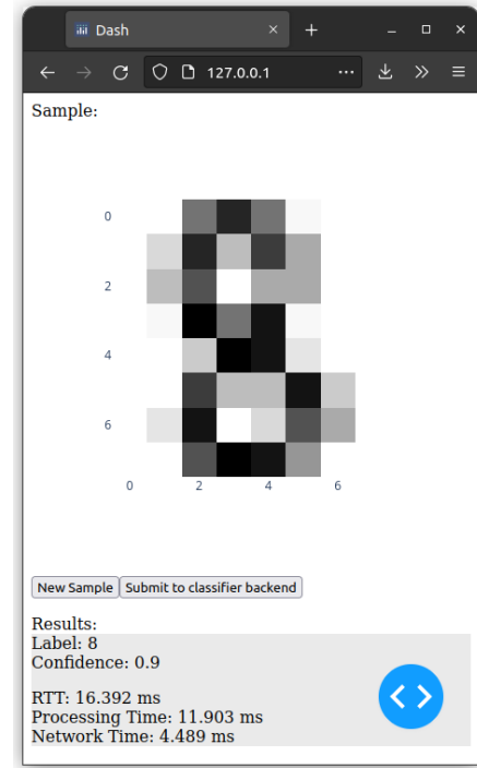
Fig. 7: Screenshot of the user interface of demo workload 1. After deciding on placement of the compute backend and the type of physical layer connecting client and backend, participants will use this interface to interact with the system.
