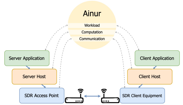
Fig. 1: Layered structure of an Ainur experiment
