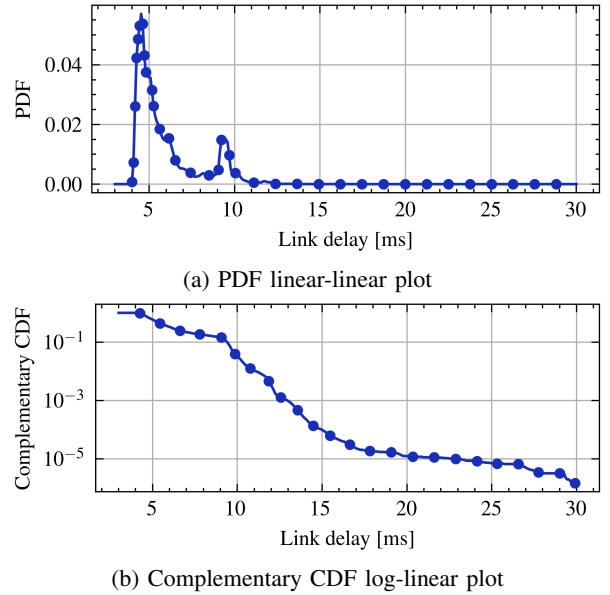
Fig. 1: Distribution of downlink latency, as observed from commercial off-the-shelf (COTS) private 5G system
