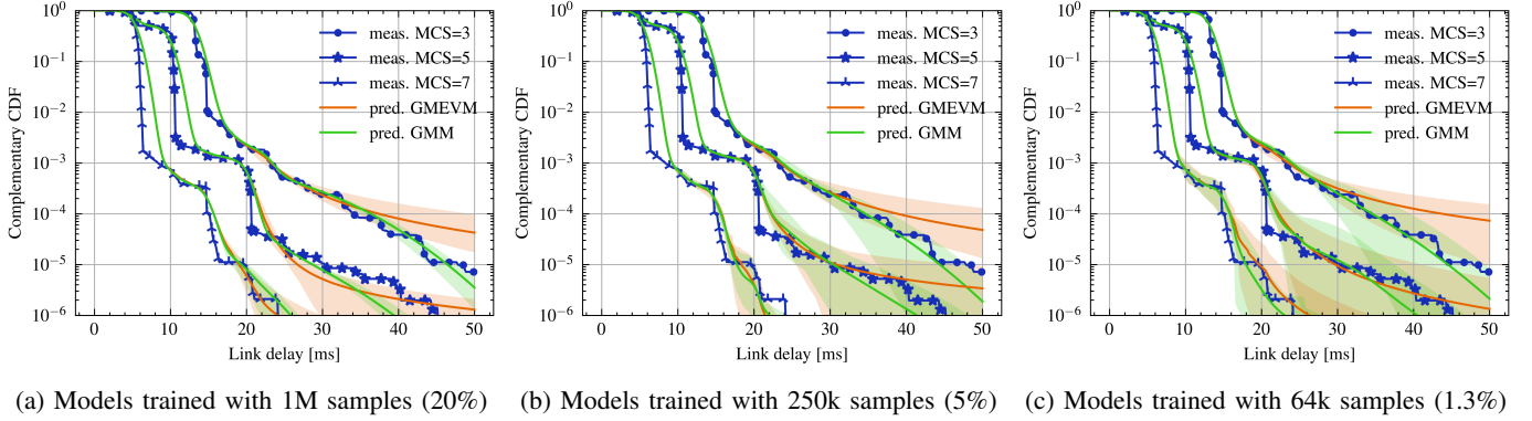
Fig. 6: SDR 5G uplink latency tail probability measurements conditioned for different MCS indices with 5M samples vs predictions of MDN models trained with different numbers of samples and added Gaussian noise
