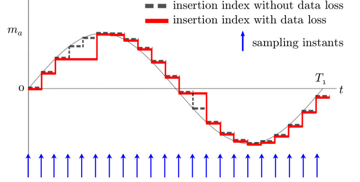
Fig. 4. Received insertion indices by the submodules with and without packet losses in wireless communication.
