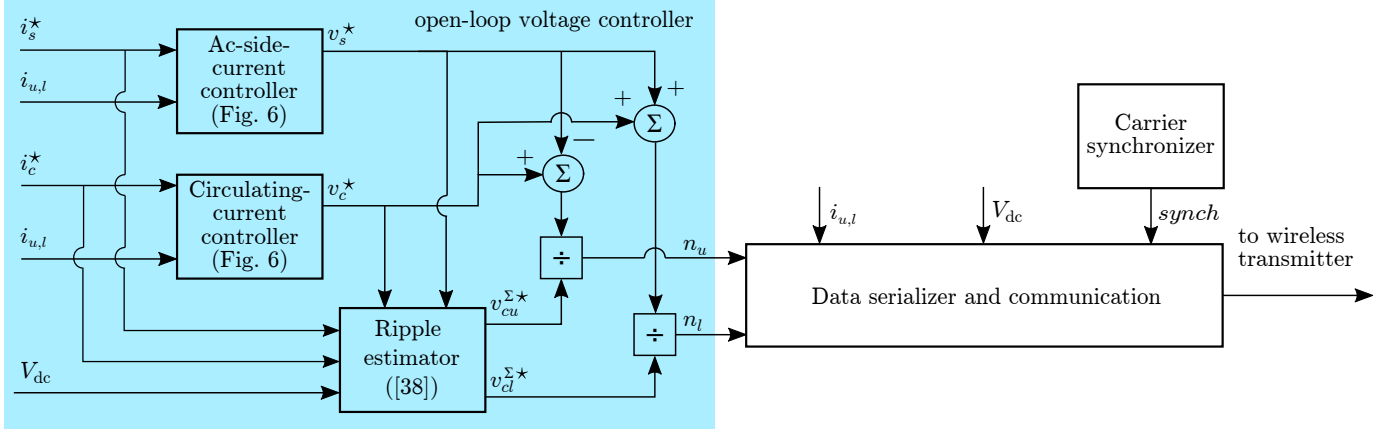
Fig. 7. Central controller block diagram of the experimental setup. i_s^* and i_c^* are calculated internally using V_{dc} and R_o that are provided by the operator, i_{u,l} are obtained from wired measurements, as shown in Fig. 5. synch is generated internally.
