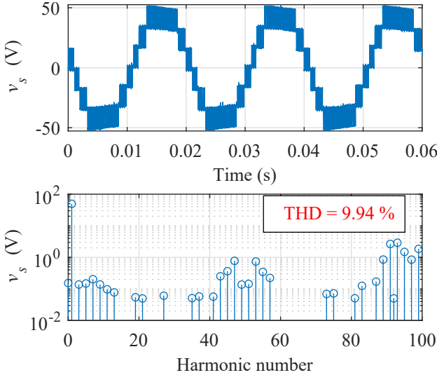
Fig. 13. Ac-side voltage (upper) and harmonics spectrum (lower). The fundamental component peak value is 49.50 V.
