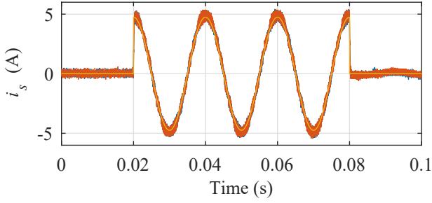
Fig. 16. Ac-side current dynamic responses of the wired (blue), wireless (orange) cases, and i_s^* (yellow) overlapped. At 0.02 s i_s^* is stepped from 0 to 4.75 A and at 0.08 s back to 0 A.
