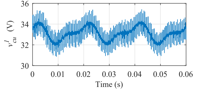
Fig. 15. Capacitor voltage of a submodule. The mean value is 33.12 V.
