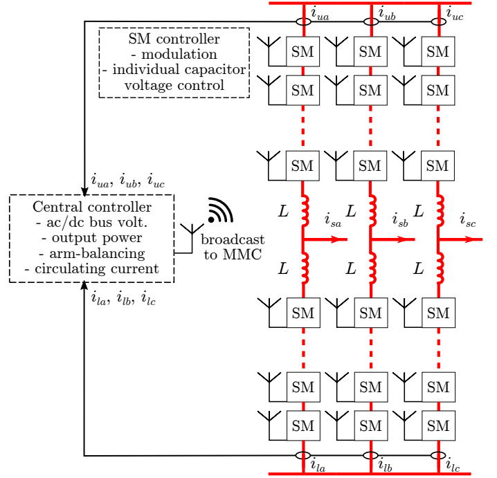
Fig. 3. The architecture of the proposed wireless MMC submodules control.
