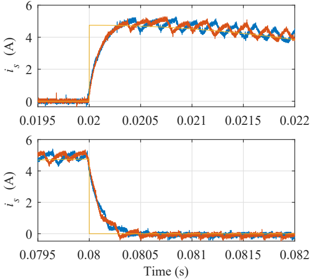
Fig. 17. Zoom-in views of the ac-side current dynamic responses of the wired (blue), wireless (orange) cases, and i_s^* (yellow) around the step times. At 0.02 s i_s^* is stepped from 0 to 4.75 A and at 0.08 s back to 0 A.
