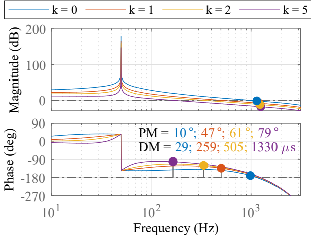
Fig. 10. Bode plot of the ac-side-current control open-loop transfer function.
