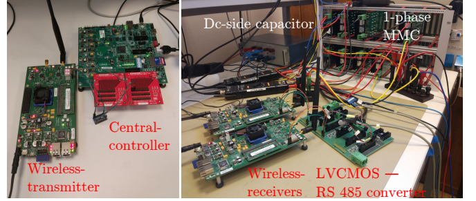
Fig. 12. Experimental setup: central controller and wireless-transmitter (left), wireless-receivers, submodules, and LVC MOS – RS 485 converter (right).
