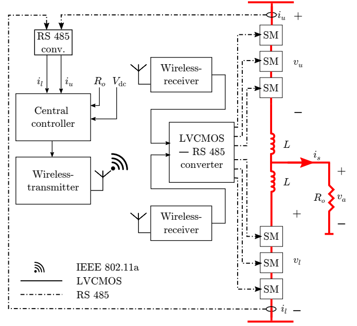
Fig. 5. Structural diagram of the wirelessly controlled single-phase MMC experimental setup. The payload of wireless packets is shown in Fig. 8. R_o and V_{dc} are provided to the central controller by the operator.
