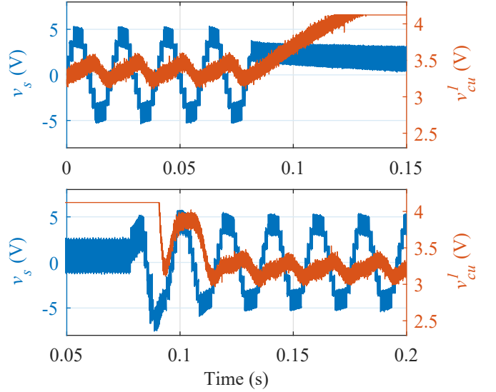
Fig. 18. Ac-side voltage (blue) and a single submodule-capacitor-voltage (orange) just before (top) and right after (bottom) two different 2.68 s single train of packet losses.
