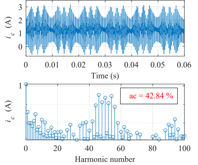
Fig. 14. Circulating current (upper) and harmonics spectrum (lower). ac value corresponds to I_{ac,rms}/I_{dc} , including all the ac harmonics. Dc is 1.25 A.
