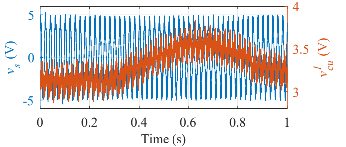
Fig. 19. Ac-side voltage (blue) and a single submodule-capacitor-voltage (orange) during a periodic train of packet losses. Every third packet is transmitted.
