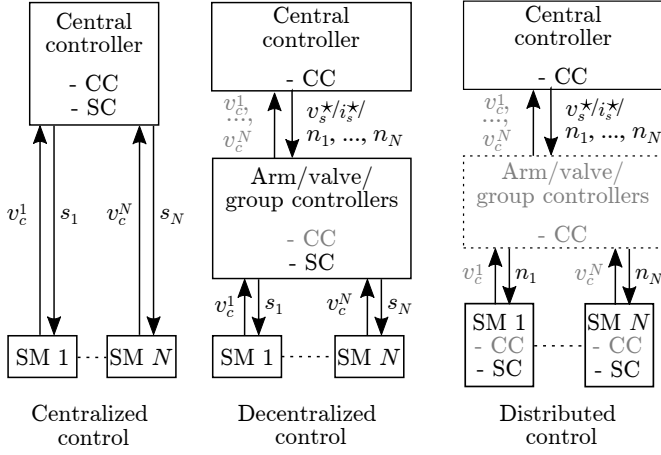
Fig. 2. The three main internal control architectures of MMCs. CC and SC stand for converter control and switching control, respectively.
