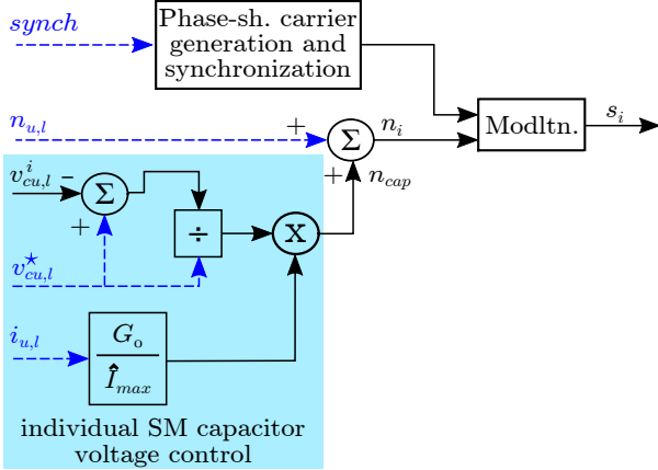
Fig. 9. Submodule controller block diagram of the experimental setup. The dashed inputs in blue are wirelessly received, v_{cu,l}^i is measured locally. v_{cu,l}^* is equal to V_{dc}/N .
