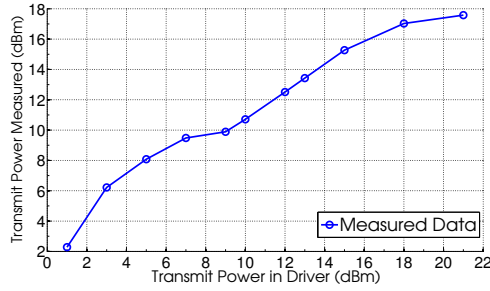
(a) Mapping the transmit power value set in software to the measured power.
