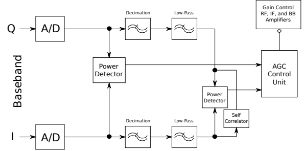
Fig. 4. Automatic gain control logic blocks [23].
