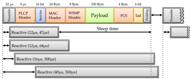
Fig. 7. Reactive jammer profiles in the time domain compared with a default 802.11p transmission.
