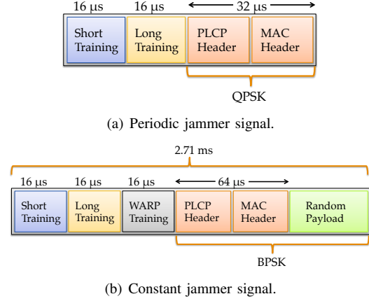
Fig. 6. Frame format of the jamming signals generated by the WARP device. Short interference signal with a 64\mu\text{s} duration (Fig. 6(a)) for the periodic jammer, and long interference signal with a 2.71 ms duration (Fig. 6(b)) for the constant jammer.
