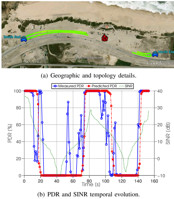
Fig. 23. Platooning movement under impact of the reactive jammer (16 \mu s, 500 \mu s) in the seafront scenario.
