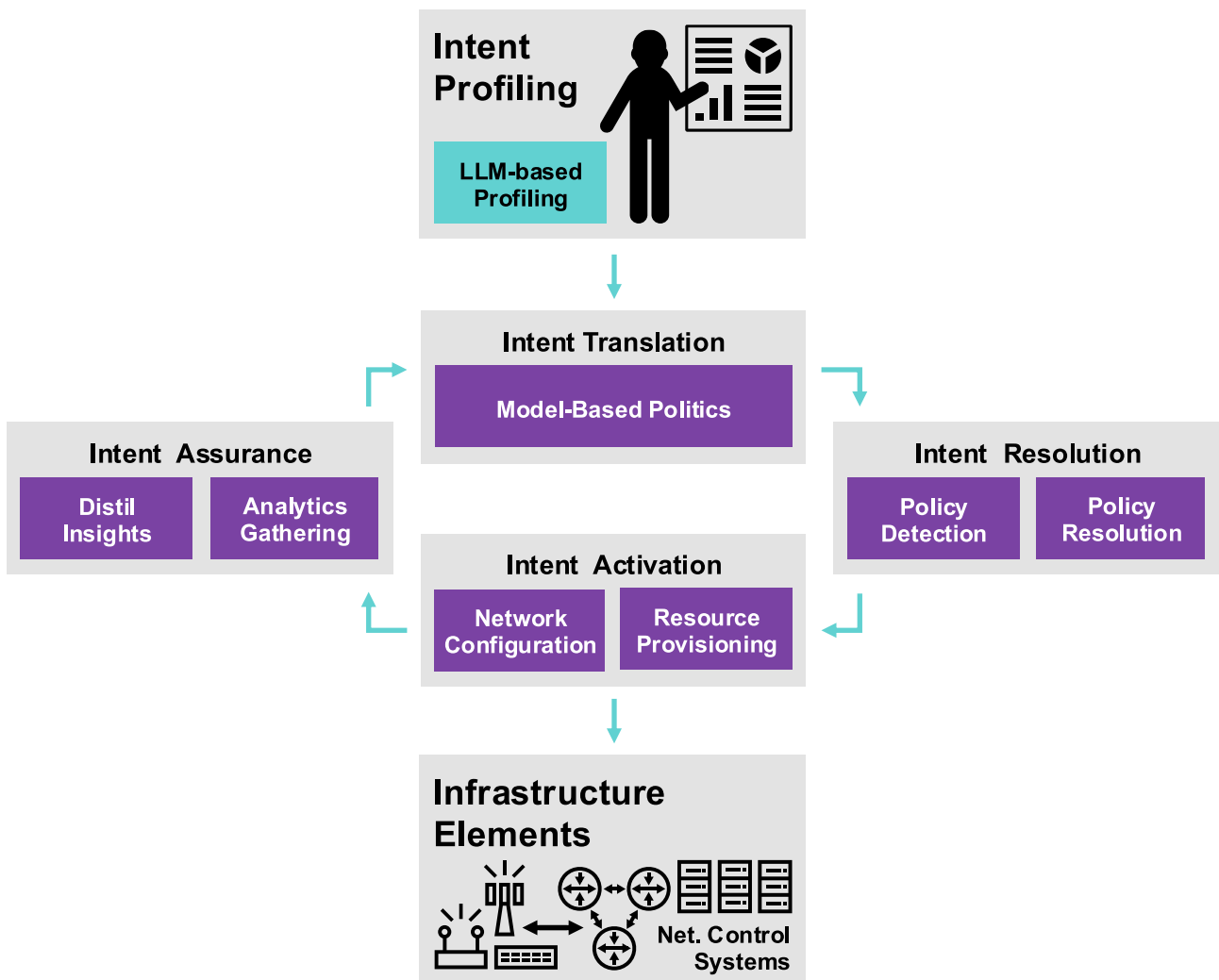
Fig. 16: Process and components of IBN.
