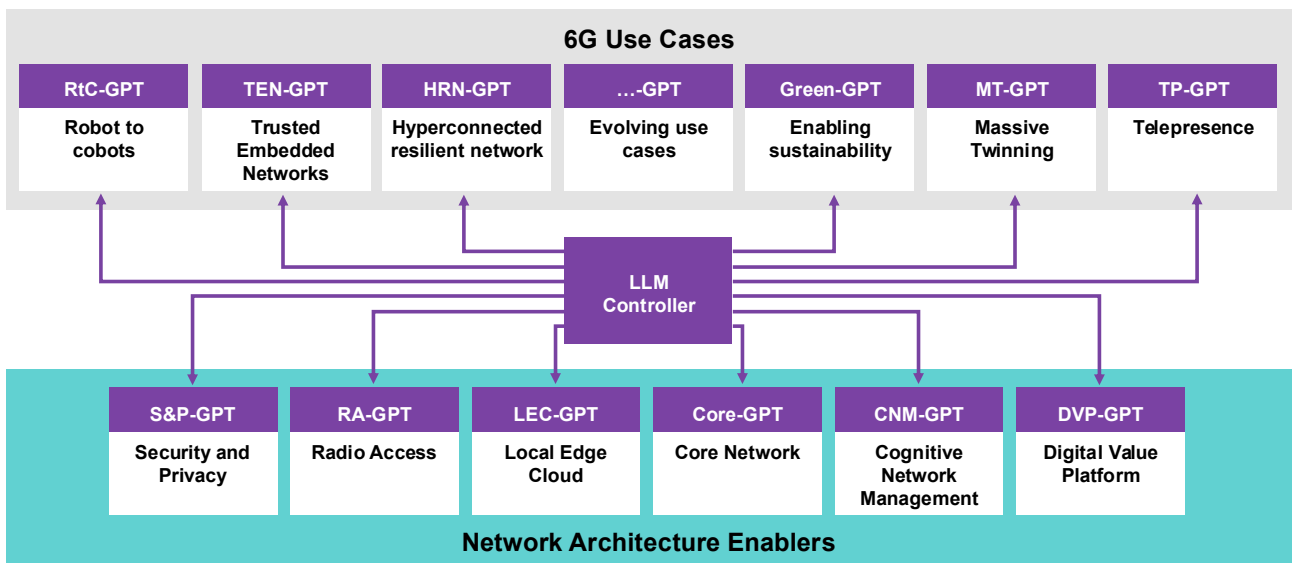
Fig. 3: Taxonomy of LLMs for 6G, mapping the potential applications of LLMs to both 6G use cases and underlying network architecture enablers. The LLM controller serves as a hub, suggesting the cooperative and management roles LLMs can play in a 6G ecosystem.
