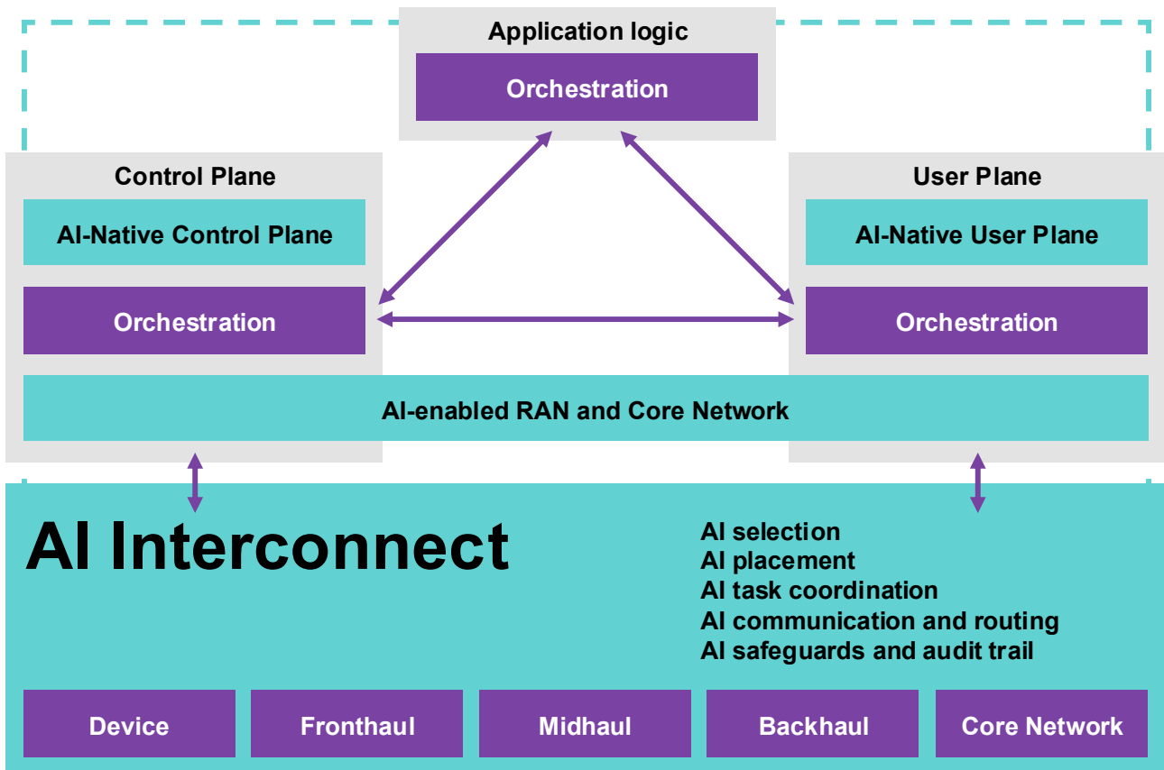
Fig. 1: AI Interconnect’s cross-layer design across control, user, and application planes.
