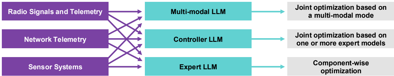
Fig. 4: Illustration of three LLM processing approaches for multimodal data. The scenarios include inputs from radio signals and telemetry, network telemetry, and sensor systems. The depicted approaches are: a multimodal capable LLM, a controller LLM for processing and result aggregation, and component-wise LLMs without aggregation.
