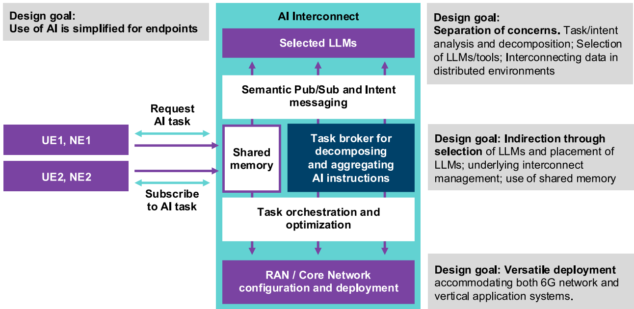
Fig. 9: GPT-Driven AI Interconnect Architecture. Our approach is structured around four pivotal design goals, from simplifying end-user interactions to ensuring versatile deployment across varied contexts, all rooted in foundational components for optimum efficiency and adaptability.
