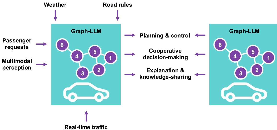
Fig. 12: Graph-LLMs for autonomous multi-agent systems
