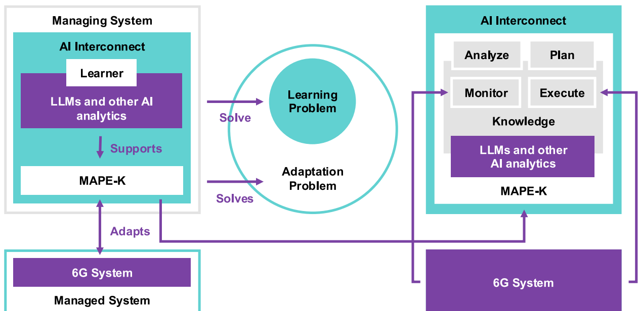
Fig. 8: MAPE-K as enabling paradigm of the AI Interconnect. On the left, relation of learning problem and adaptation problem with the components of the managing system. On the right, structure of an autonomous element. Elements interact with other elements and with human programmers via their autonomic managers.
