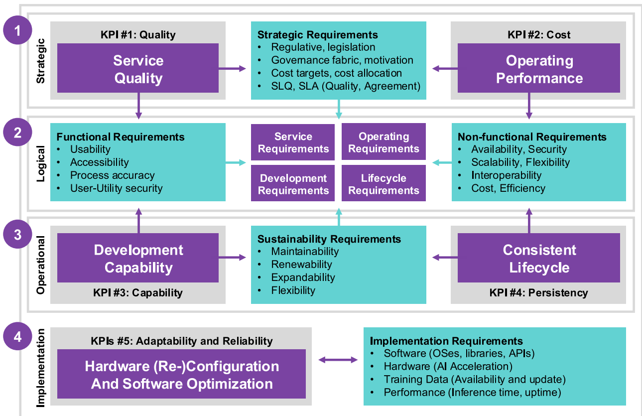
Fig. 6: A holistic representation of the 6G architectural framework, illustrating the layered approach from high-level strategic objectives to practical implementation considerations. This framework integrates LLM and GPT technologies across strategic, logical, operational, and implementation layers, with associated key performance indicators (KPIs) and requirements.
