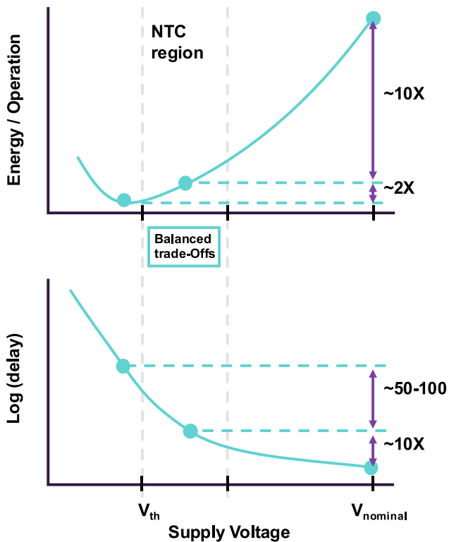
Fig. 13: Impact of voltage down scaling on energy efficiency and logic delay (adapted from [200] © IEEE).
