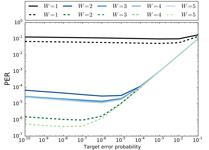
Fig. 2. PER for an increasing number of hops ( W ) varying the target error probability \epsilon^* . For solid lines the avg. link quality is \bar{\gamma} = 5 dB, while for dashed lines the avg. link quality is \bar{\gamma} = 7.5 dB.
