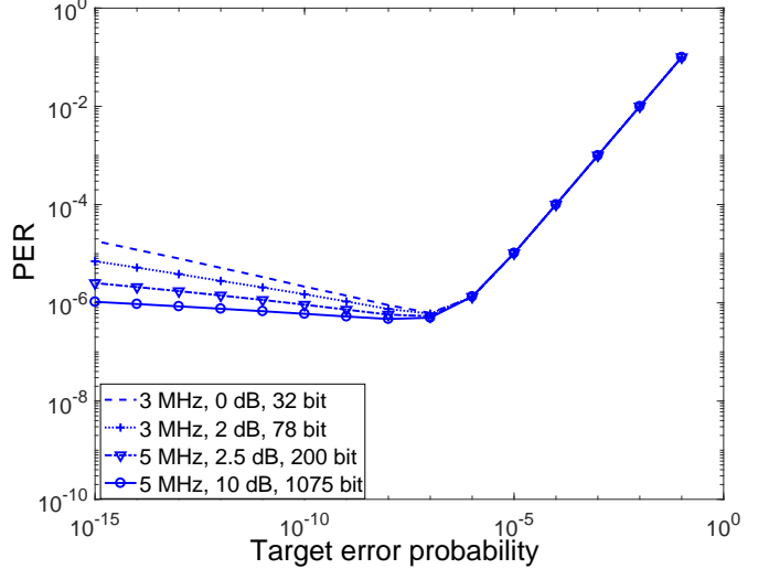
Fig. 6. PER of 4 Antenna for different channel bandwidths, SNRs, and packet sizes varying the target error probability \epsilon^* .
