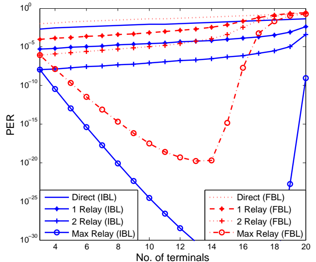
Fig. 8. The achievable PER at the optimal choice of target error probability while varying the number of terminals N for BEST-RELAY.
