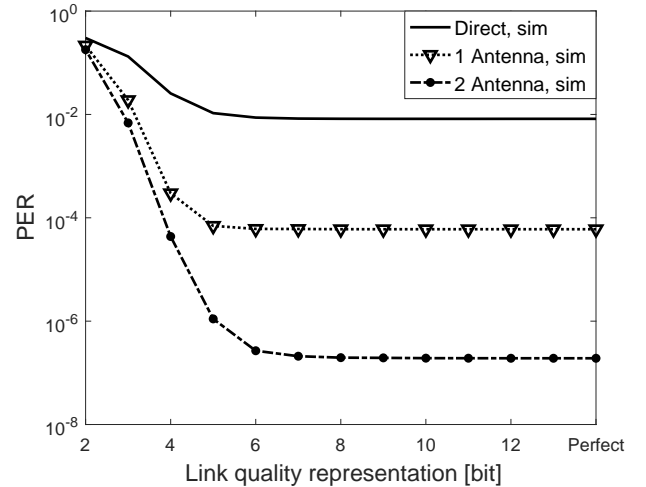
Fig. 4. PER depending on the quantization of link qualities. We vary the number of bits used to represent a single link quality, where perfect is the reference for an arbitrarily high representation.
