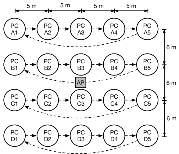
Fig. 10. Example topology for industrial automation scenario.
