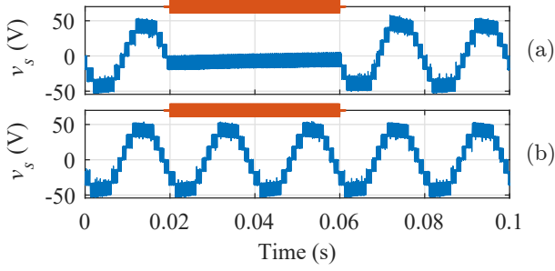
Fig. 8. Ac-side voltage with the existing (a) and the proposed (b) control method.
