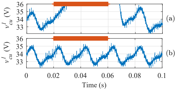
Fig. 10. Capacitor voltage of a submodule with the existing (a) and the proposed (b) control method.
