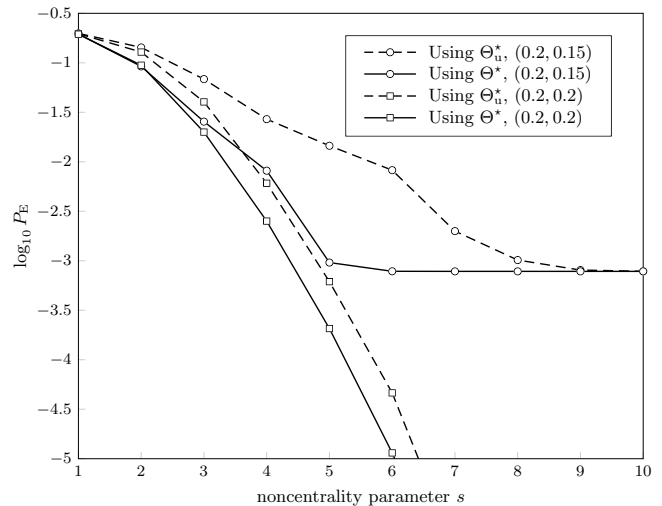
Fig. 4. Error probability performance of a network of N = 4 unlimited-capacity battery energy harvesting sensors while using unconstrained \Theta_u^* and adapted \Theta^* thresholds and for different (\pi_1, p_e) .
