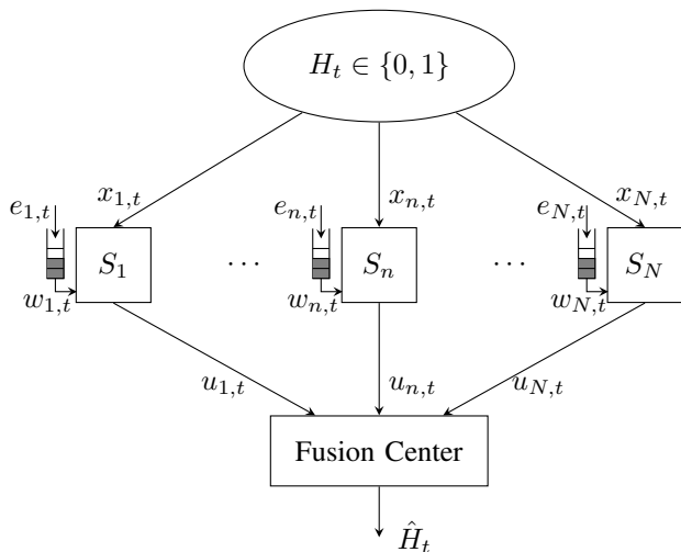
Fig. 1. Decentralized detection in energy harvesting parallel network.
