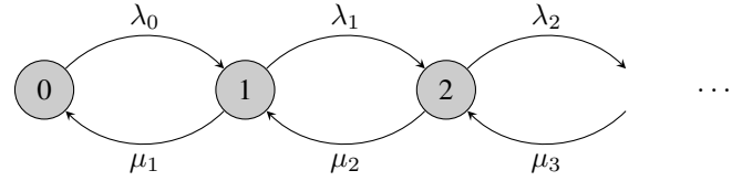
Fig. 2. A birth-death process.
